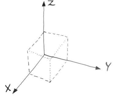
Figure 4.3: Illustration of euclidean space.
