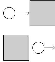
Figure 5.4: Illustration of x \rightsquigarrow y respective x \leftarrow y
