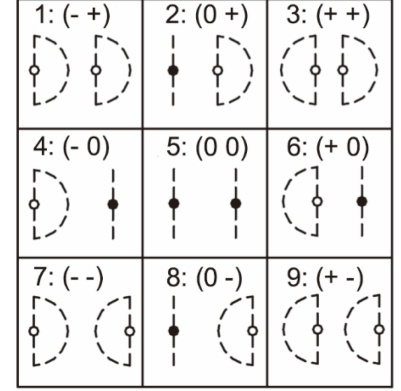
Figure 4.2: The relationship between moving objects in QTC [Chavoshi et al., 2015].
